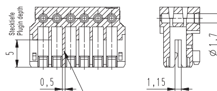
Codiersteg (z.B. zwischen Kammer "4" und "5") Solid wall (e.g. between chambers "4" and "5")
